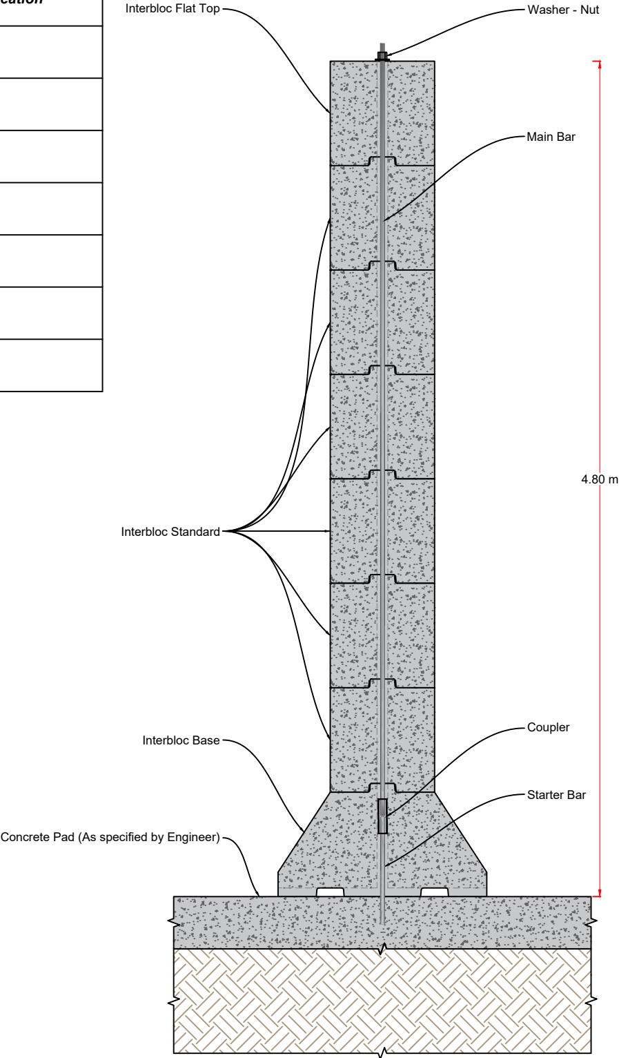
INTERBLOC® Bunker Wall Cross Section Vertical Reinforcing - Standard Kits
