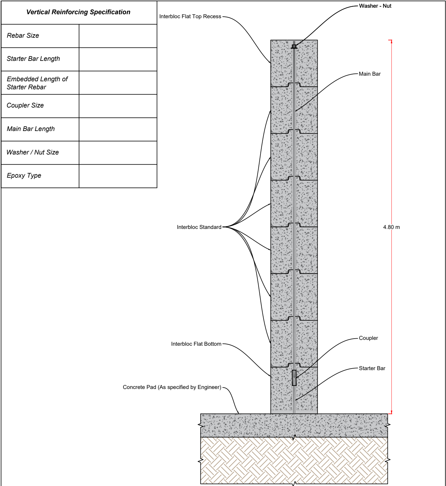
INTERBLOC® Bunker Wall Cross Section Vertical Reinforcing - Standard Kits
