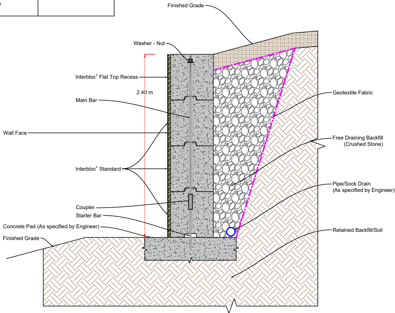
INTERBLOC + ® Retaining Wall Cross Section Vertical Reinforcing - Standard Kits
