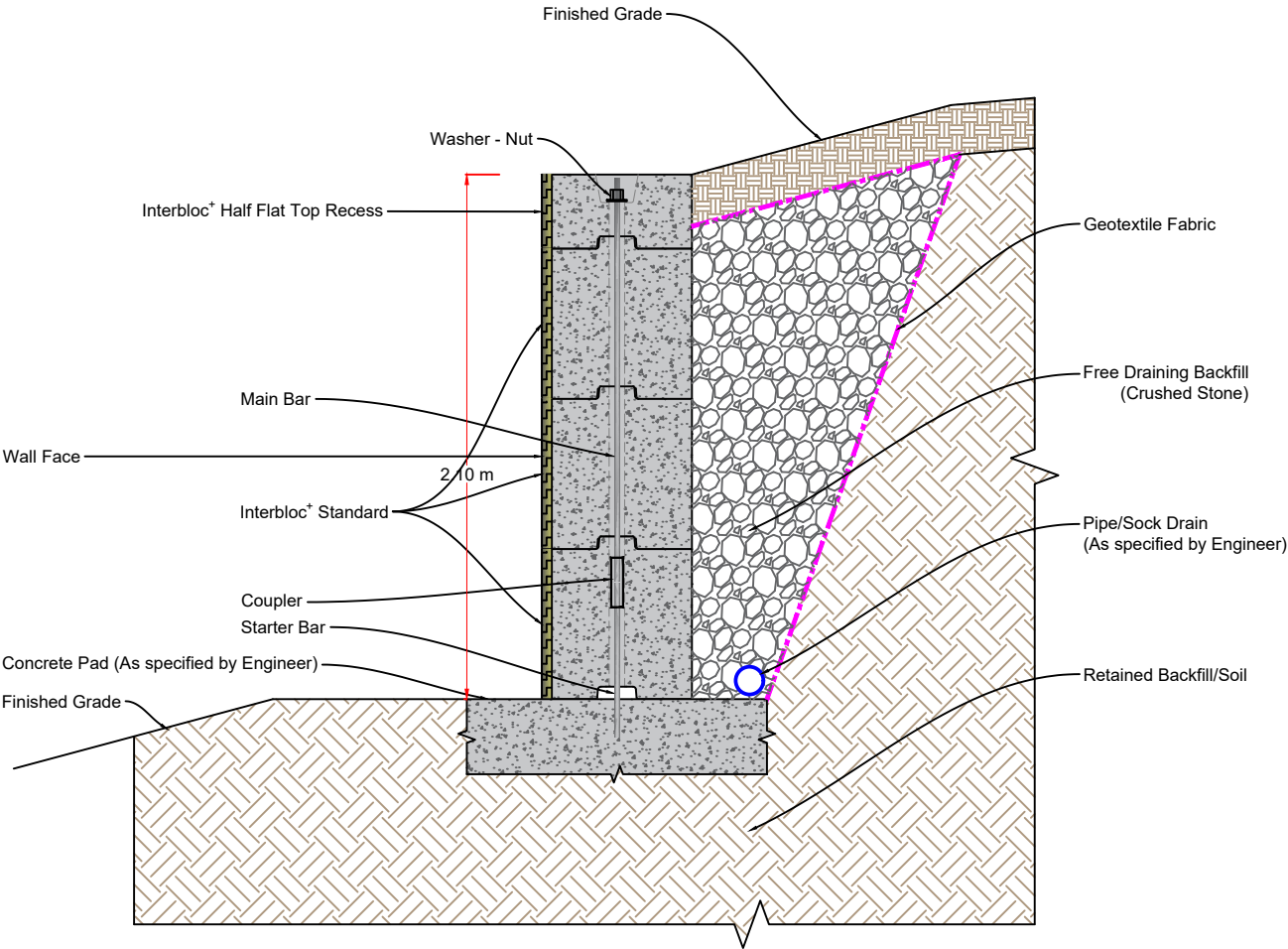
INTERBLOC+® Retaining Wall Cross Section Vertical Reinforcing - Standard Kits
